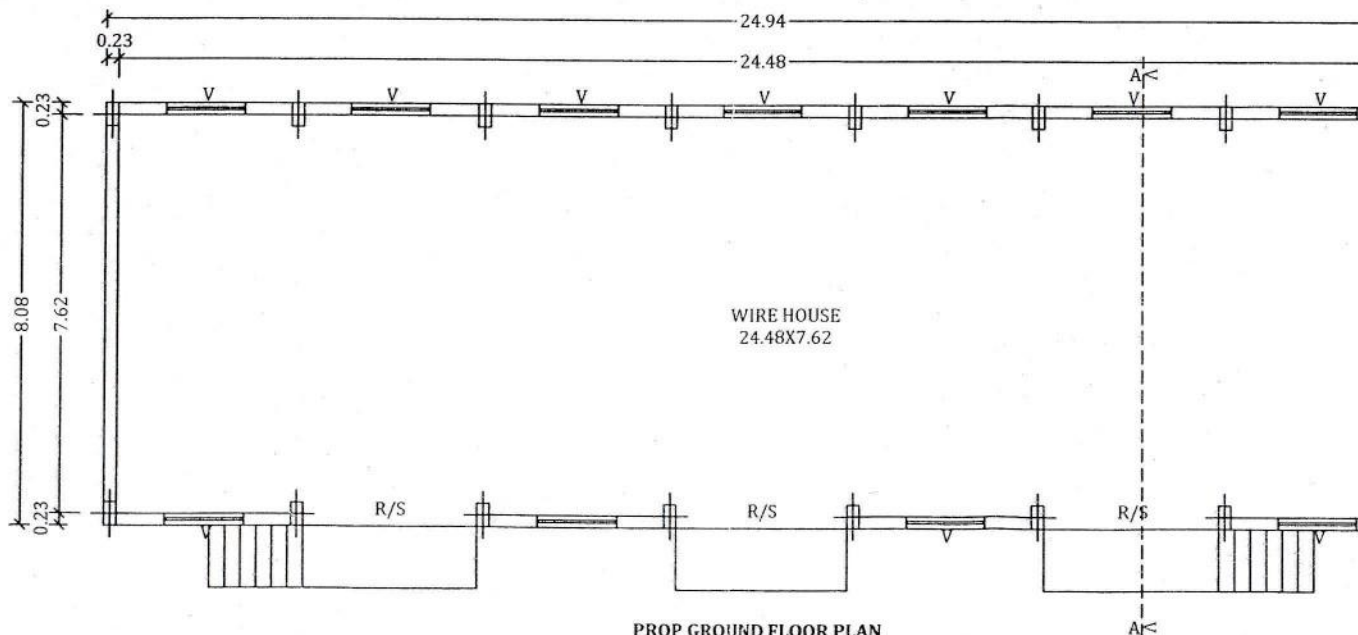
PROP GROUND FLOOR PLAN SCALE 1:100
