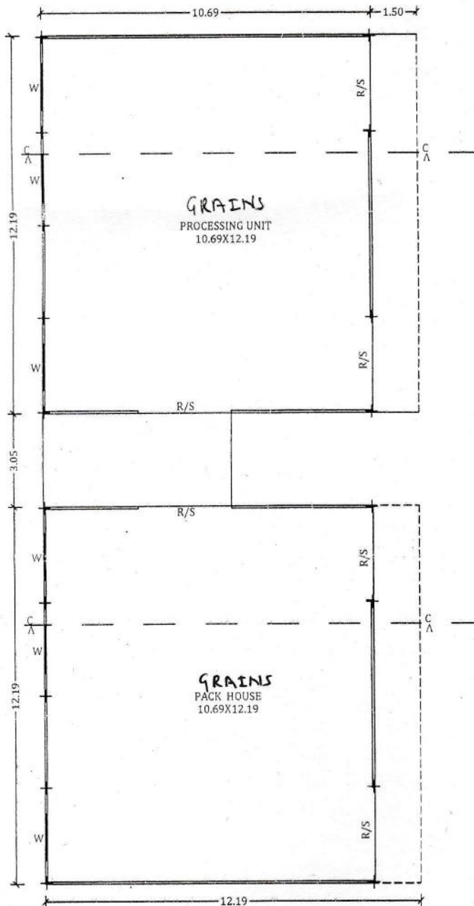
GROUND FLOOR PLAN ③ SCALE 1:100
